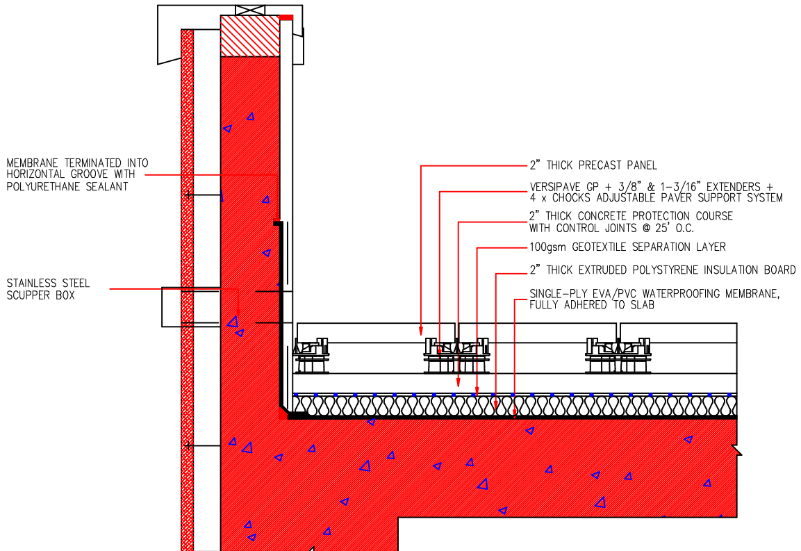
ROOF PARAPET DETAIL
