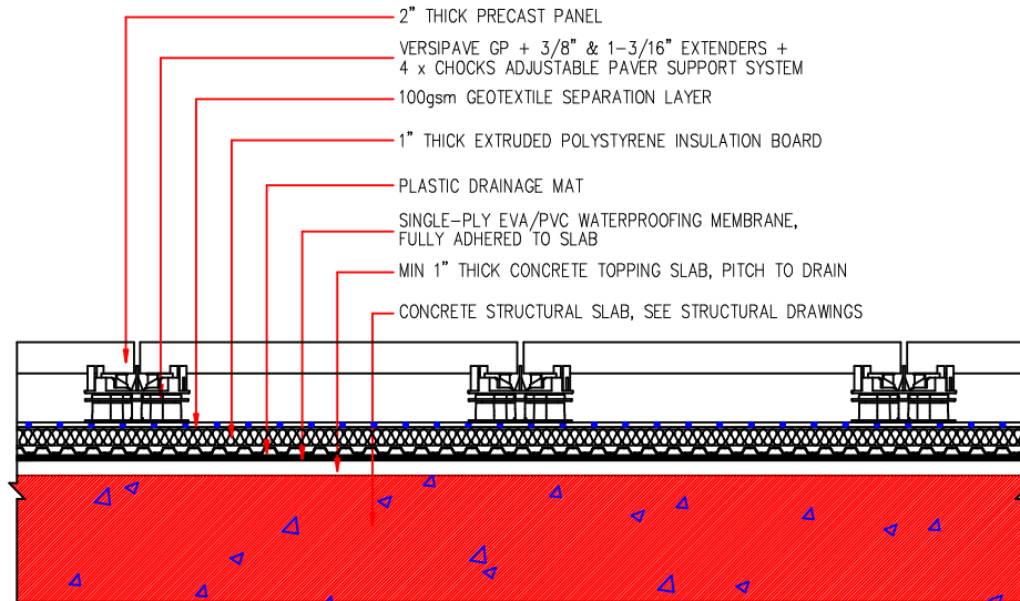
ROOF TERRACE DETAIL
