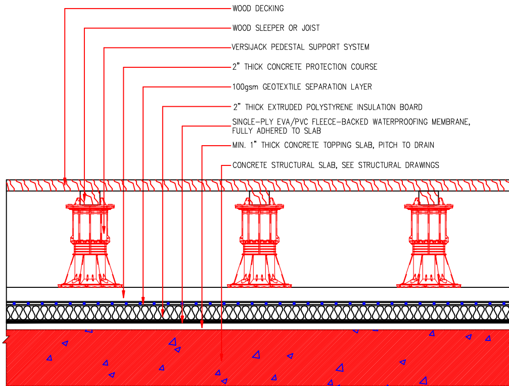
VERSIJACK S SECTION DETAIL (TIMBER DECK)
